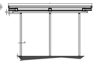
Vista frontale (3 profili guida) Frontal view (3 guide profiles)
