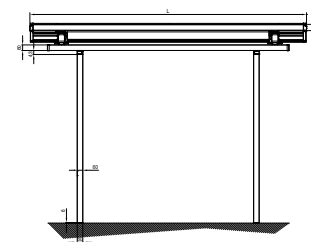
Vista frontale (2 profili guida) Frontal view (2 guide profiles)
